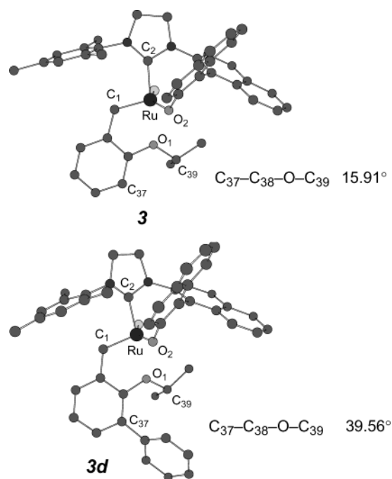
Figure 2. X-ray crystal structure of chiral Ru complex 3 and 3d .
