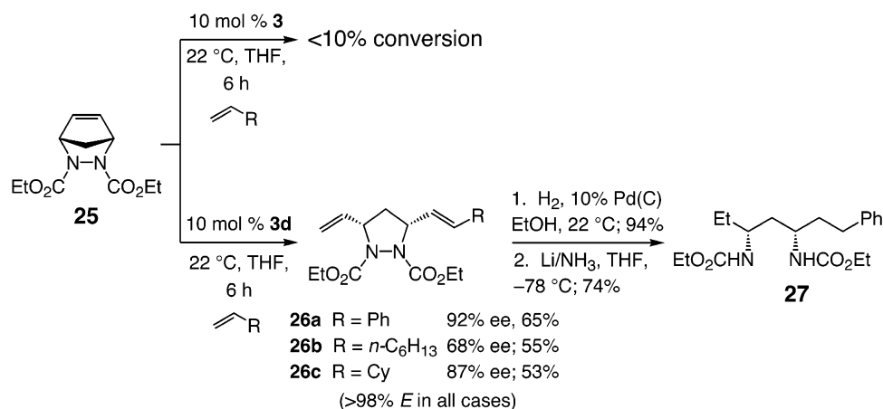
Scheme 3. Ru-Catalyzed ARCM Reactions
