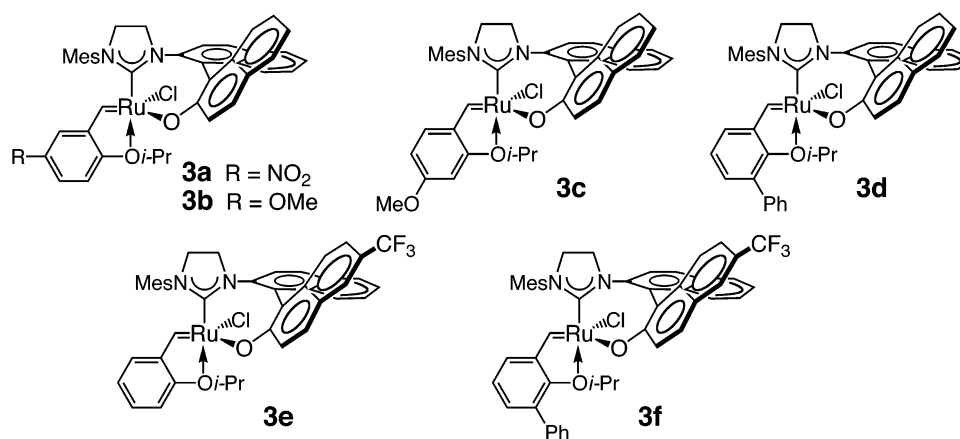
Chart 2. Second Generation Chiral Ru-Based Metathesis Catalysts Bearing Styrene Ether Ligands
