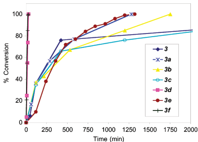
Figure 1. Relative rates of AROM/CM reactions (to afford 11a ) catalyzed by various chiral Ru catalysts (22 °C). (Reactions with catalysts 3 and 3c require 4000 min to proceed to >98% conv).
